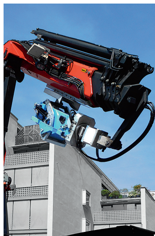
Pick up device incl. Swing break and a radio crane weighter.
